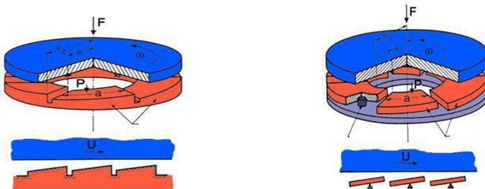
Fig.1.6a Fixed-incline-pads thrust bearing
