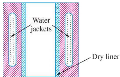
a) Dry liner.
