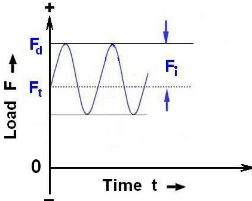
Fig. Dynamic loading on gear F = F_t + F_d
