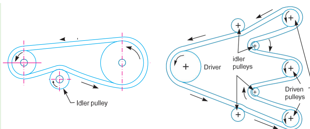
1. Belt drive with single idler pulley. (b) Belt drive with many idler pulleys.
