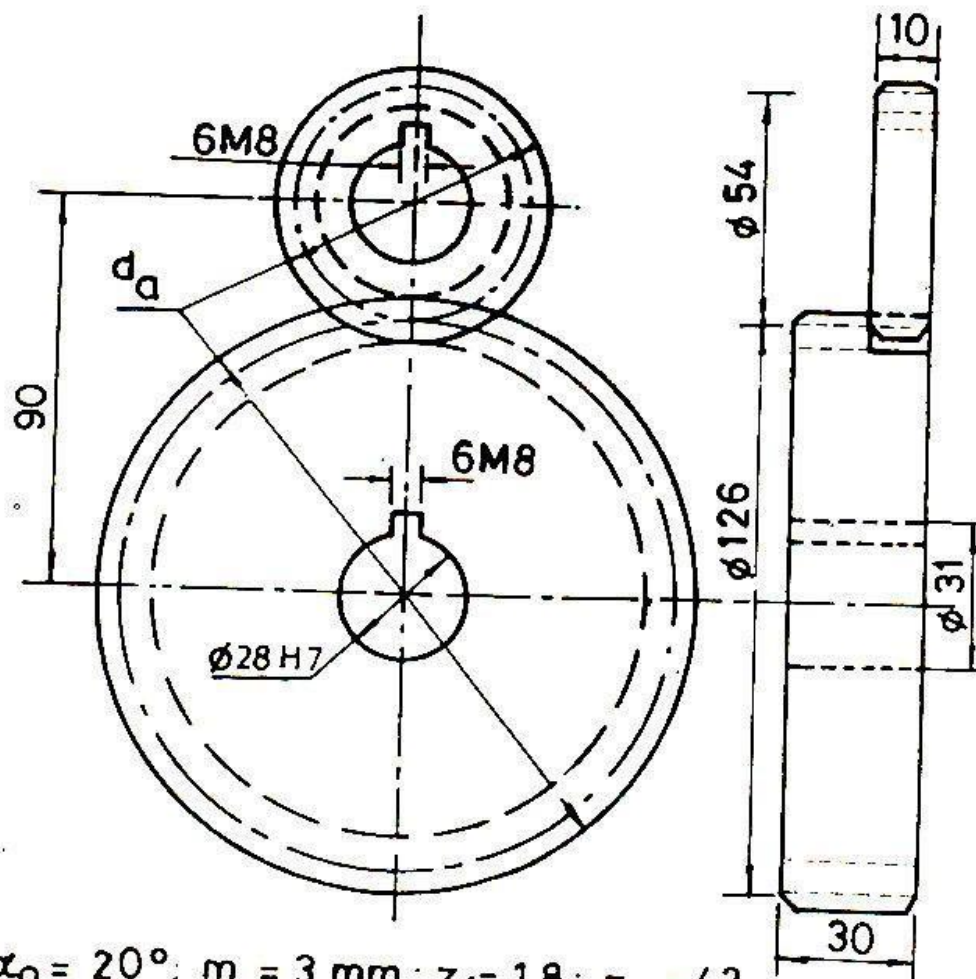
Gear Set
