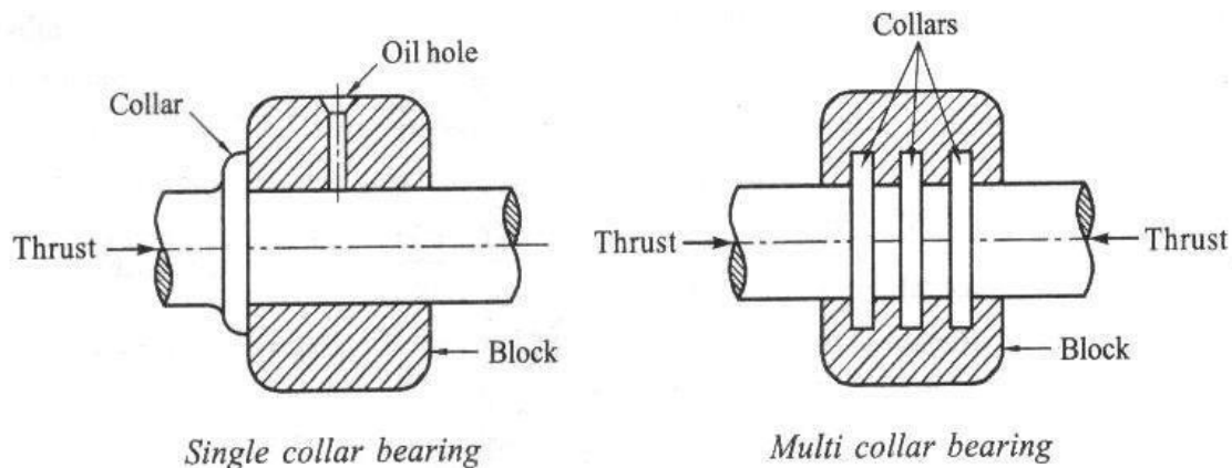
Fig.1.5 Collar bearings
