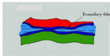
Fig.1.11 Boundary Lubrication
